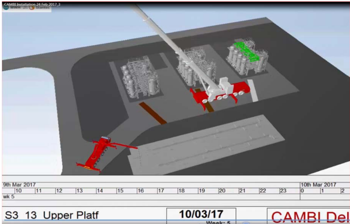
Fig 2 Final Installation sequence on Synchro identifying opportunity for concurrent working
